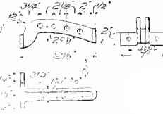
Figs. 4900-2. DEAD-LEVER STOP.
